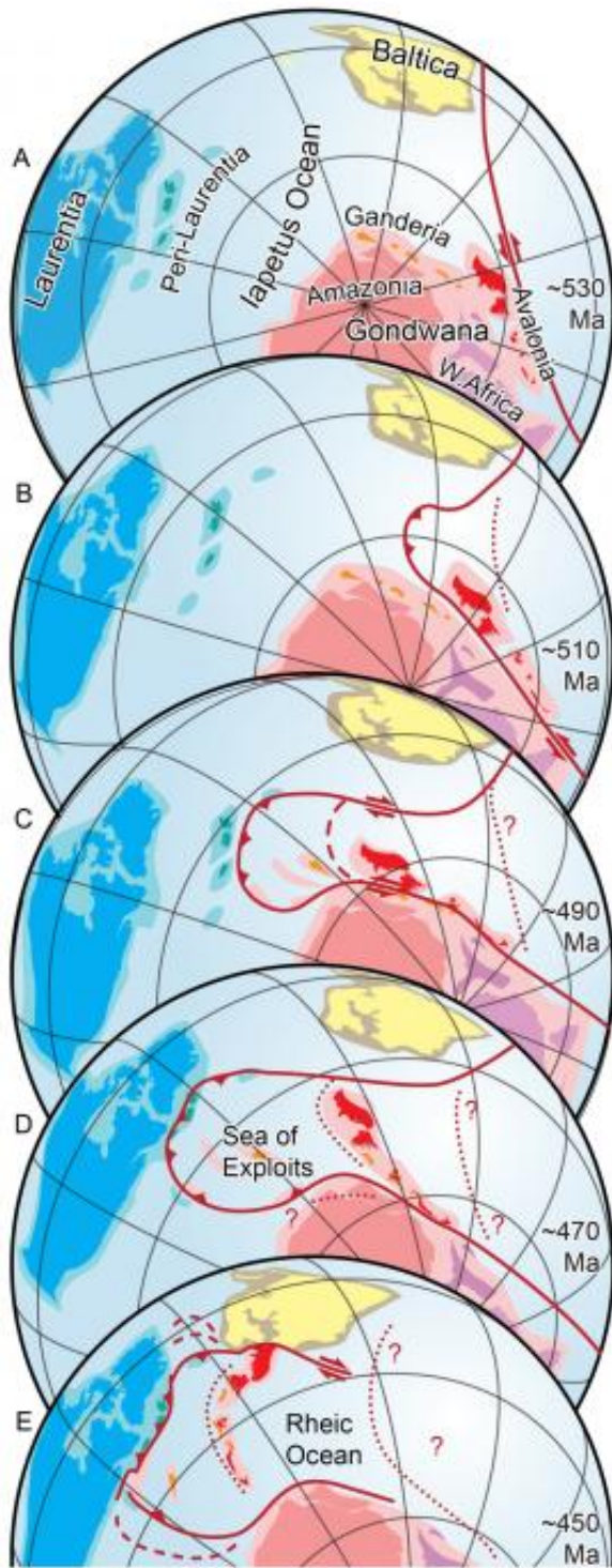
This graphic shows the possible geography of the Iapetus Ocean in a series of snapshots from the Cambrian Period (about 530 million years ago) until the Late Ordovician Period (about 450 million years ago). The continent Laurentia, which formed the core of modern North America, is shown in blue. Yellow colours
